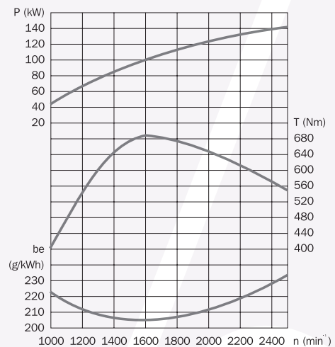
➔ BF6L 913C
